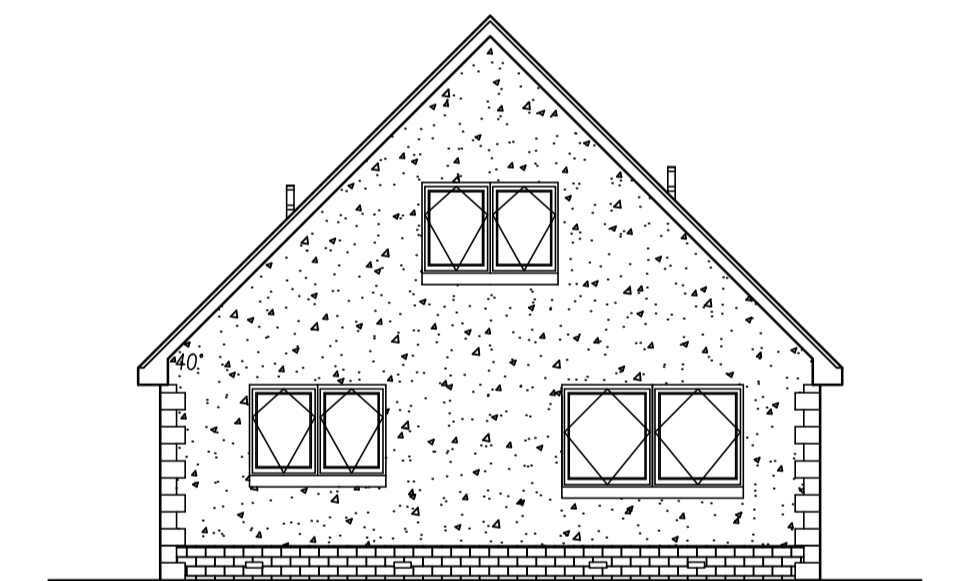
FRONT ELEVATION
