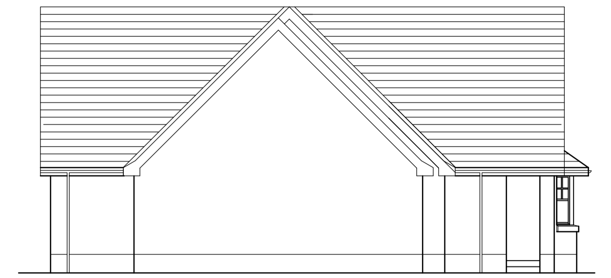
SIDE ELEVATION
