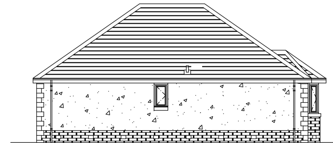
SIDE ELEVATION
