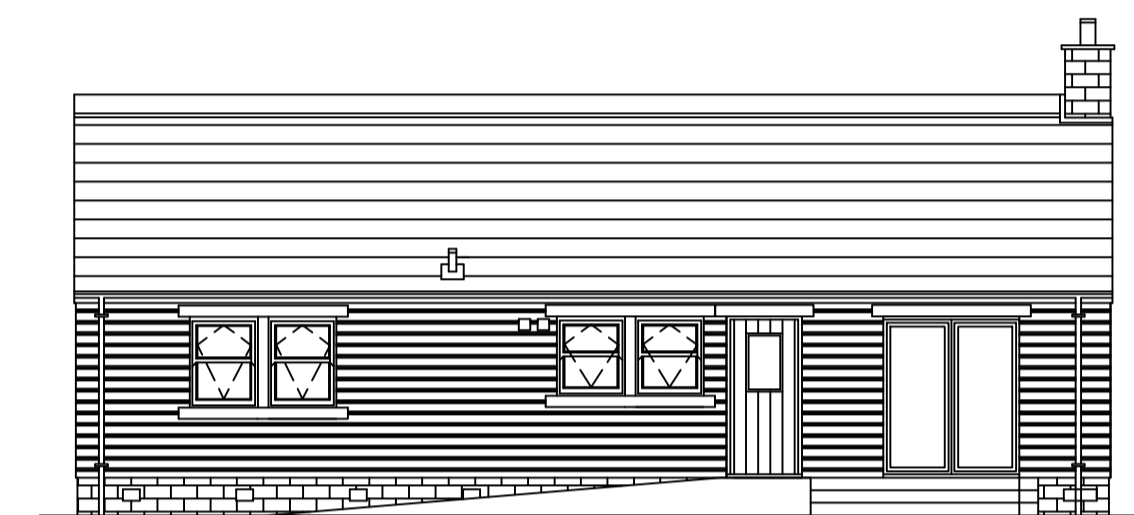
REAR ELEVATION
