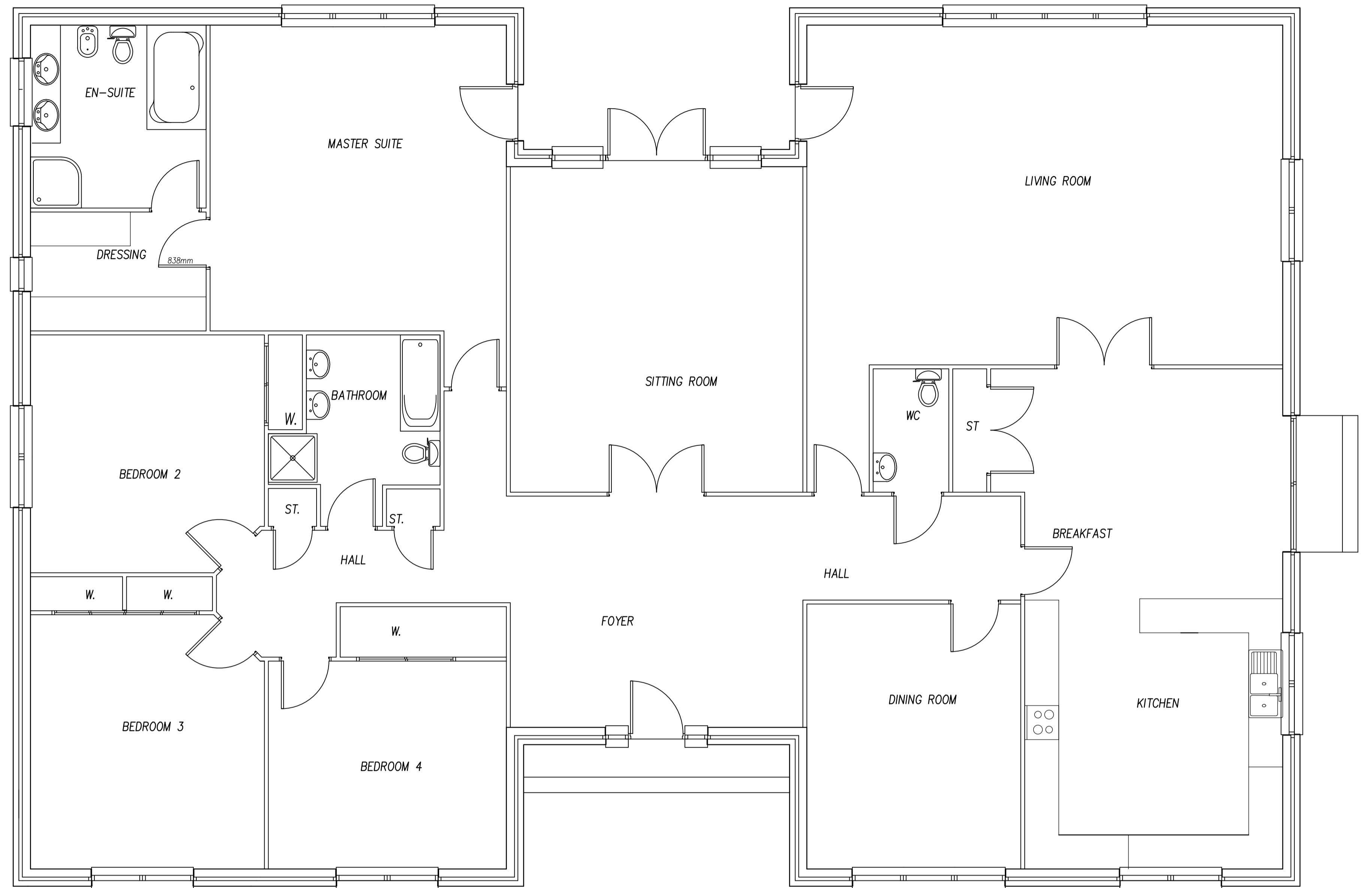
FLOOR PLAN
